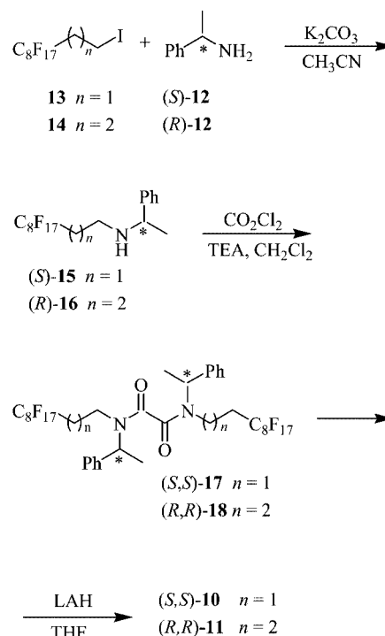
Scheme 1. Synthesis of diamines (S,S)- 10 and (R,R)- 11
