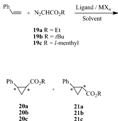
Scheme 2. Cyclopropanation of styrene with \alpha -diazoacetates
