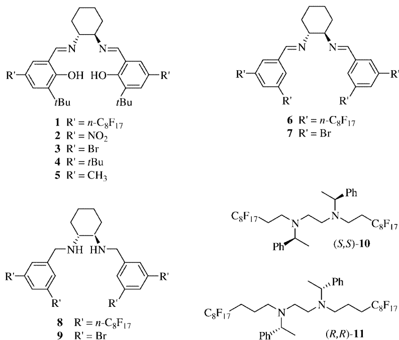
Figure 1. Ligands tested in the asymmetric cyclopropanation of styrene
